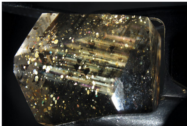
Figure 15. The changing direction of the rays is visible here when the stone is viewed through the same polished face but tilted to a slightly different orientation. Photomicrographs by Rosie Young; field of view 19.27 mm.
