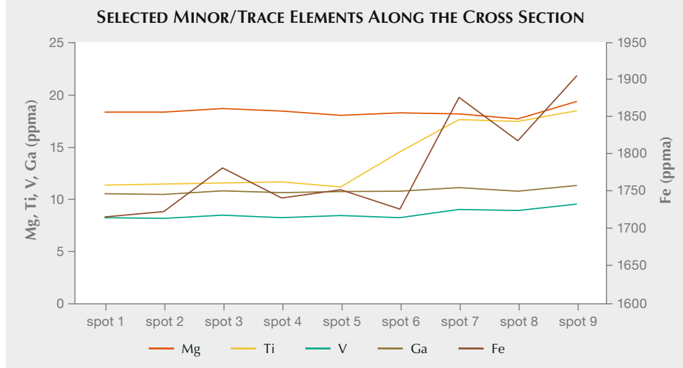
Figure 22. Sample A shows strong two-direction lamellar twinning structures (top left) and contains numerous reflective inclusions near the rim (top right). Both photos are under fiber-optic illumination; the light source of the top right photo is in a specific direction to show the reflective inclusions. Photomicrographs by Yuxiao Li; field of view 19.5 mm. The plot at the bottom shows the minor/trace element concentrations of each spot. The spot position is shown in the top right photo.
