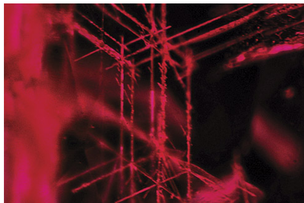
Figure 11. Rose channels in a 0.5 ct ruby. Photomicrograph by Aamir Sayed; field of view 0.75 mm.
