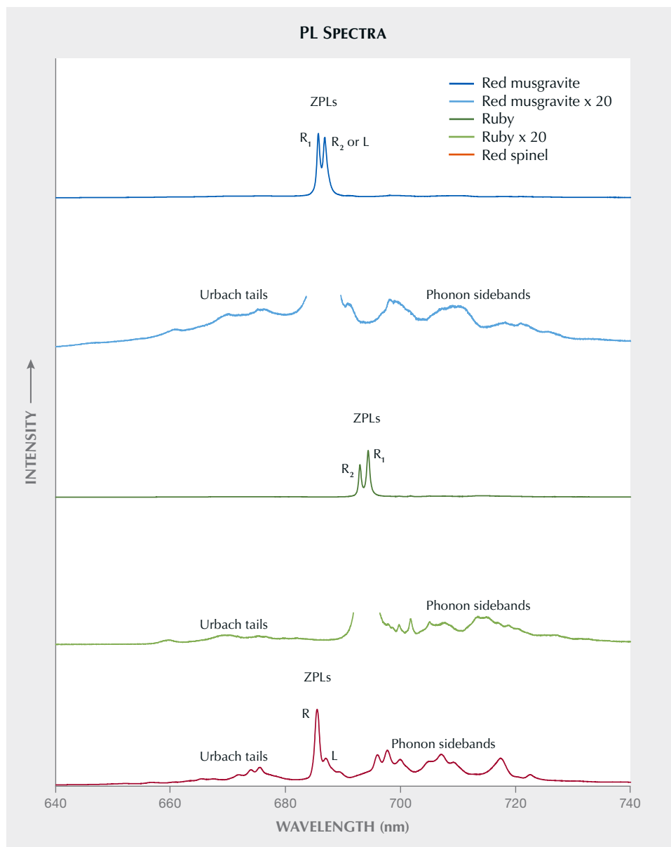
Figure 10. The PL spectrum of the red musgravite consisted of two very strong peaks at 685.7 nm ( R_1 ) and 686.8 nm ( R_2 or L ). In the spectrum below that, its weak side peaks are expanded by multiplying the intensity by 20. They are partially similar to those of ruby (692.9 ( R_2 ) and 694.4 ( R_1 ) nm), its expanded weak side bands, and a red spinel (685.5 ( R ) and 687.1 ( L ) nm). Spectra are offset vertically for clarity.
