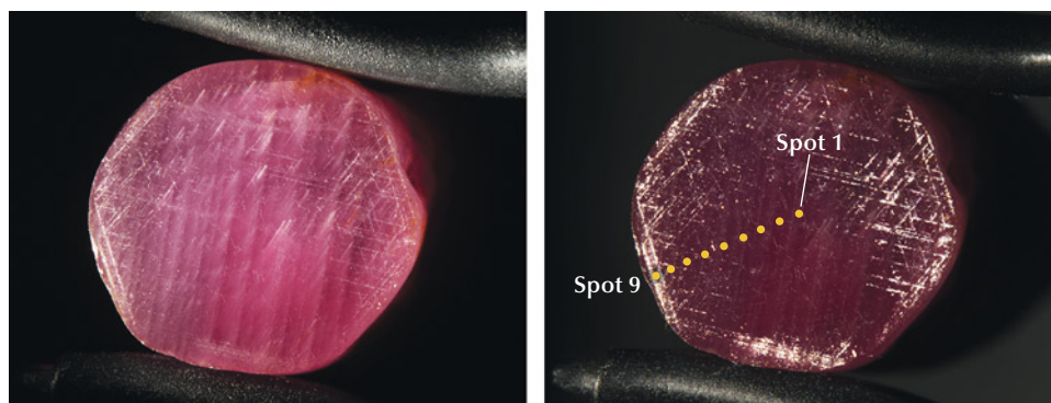
Figure 22. Sample A shows strong two-direction lamellar twinning structures (top left) and contains numerous reflective inclusions near the rim (top right). Both photos are under fiber-optic illumination; the light source of the top right photo is in a specific direction to show the reflective inclusions. Photomicrographs by Yuxiao Li; field of view 19.5 mm. The plot at the bottom shows the minor/trace element concentrations of each spot. The spot position is shown in the top right photo.
