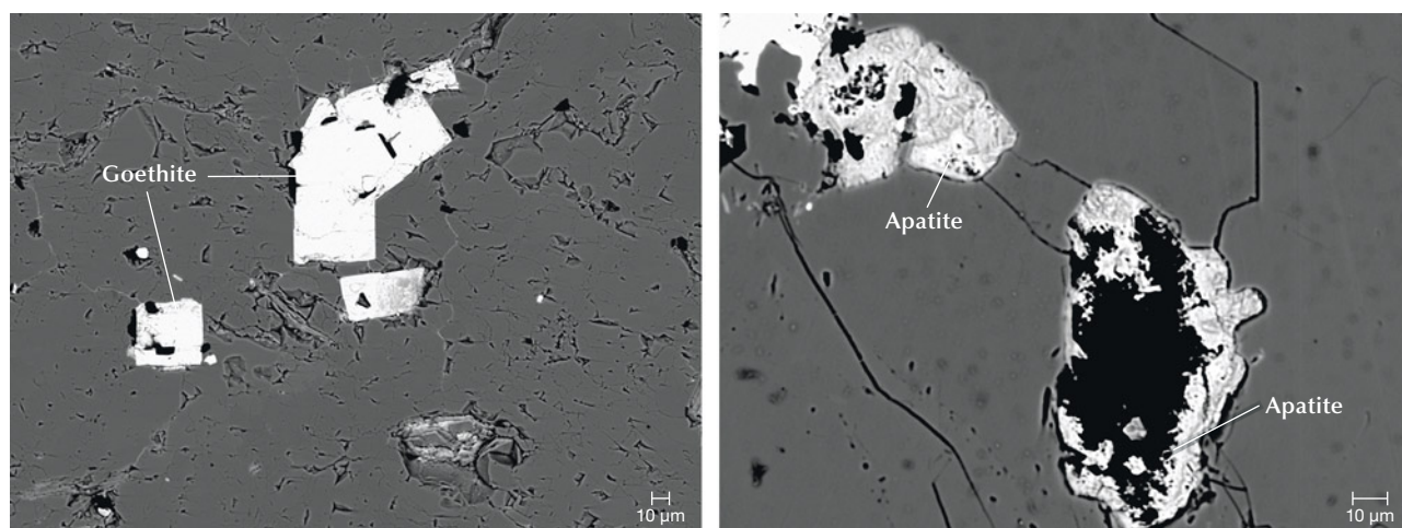
Figure 22. The occurrence of goethite and diagenetic apatite in the Tianhu East rocks, revealed in EPMA-BSE images. A: Goethite with pseudomorph cubic forms produced by the oxidation of pyrite. B: The remaining dissolved apatite exhibits incomplete shapes with numerous cavities.
