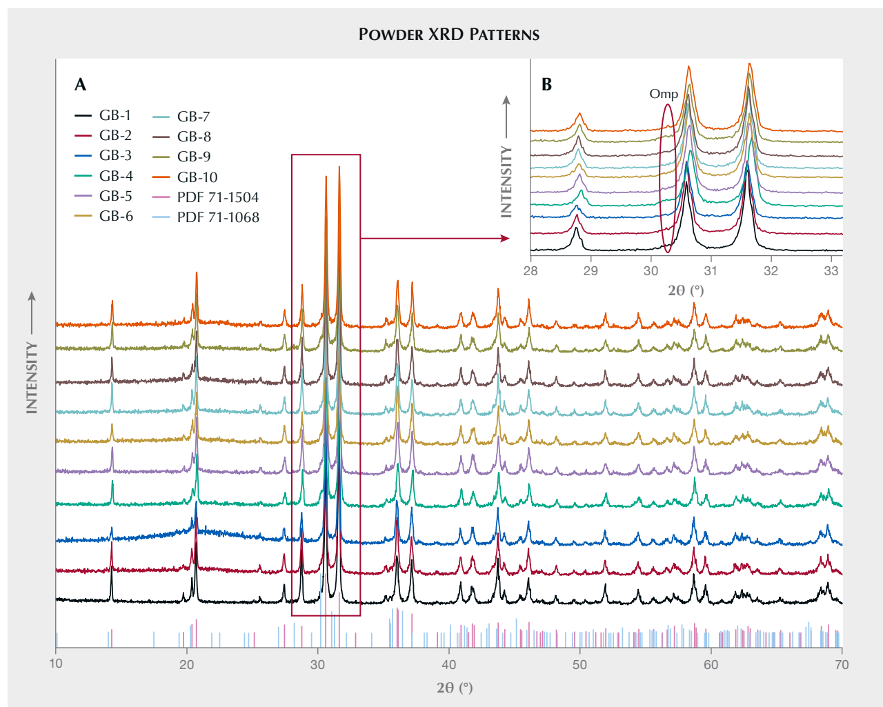
Figure 6. Powder XRD patterns of Guatemalan “ice jade” samples. The patterns are stacked for clarity. A: Almost all the diffraction peaks fit with jadeite standard diffraction peaks (ICDD PDF 71-1504). B: Matching with ICDD PDF 71-1068 reveals that a weak peak at d_{-221} = 2.952\text{\AA} ( 2\theta = 30.34^\circ ) belongs to omphacite (Omp).
