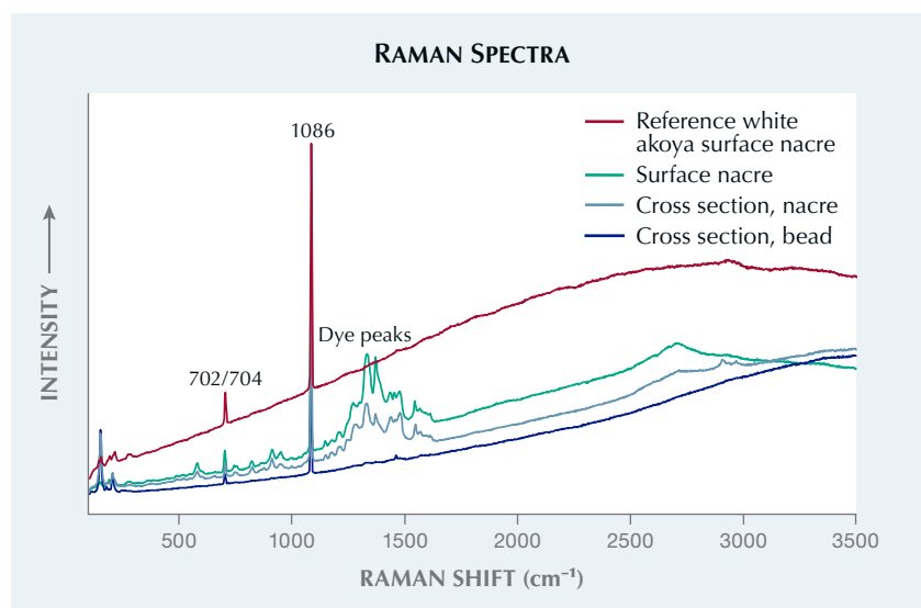
Figure 26. Raman spectra of one sample's surface nacre, nacre on the cross section, and bead nucleus, along with the surface nacre of a white akoya pearl for comparison. Unusual peaks were found in both nacre areas but not on the bead nucleus. Also shown are typical aragonite features at 702, 704, and 1086 \text{cm}^{-1} .
